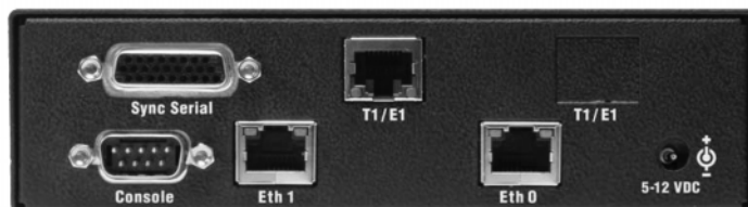
Rear Panel
