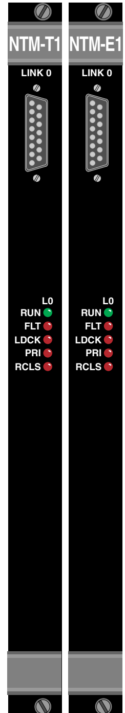
Figure 1: Front Panel Features of Xedge NTM-T1 or NTM-E1
